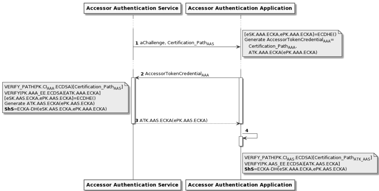
Figure 9.3: Secure SCL security protocol shared secret initialization
